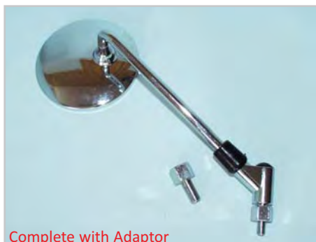
SUZUKI MR217 O.E No L/H: 56500-22010/11/45640 O.E No R/H: 56500-22010/11/45640 TYPE: Convex HEAD: Chrome STEM: Chrome FITTING: Handlebar THREAD: 8/10mm FIXING CENTRE:
