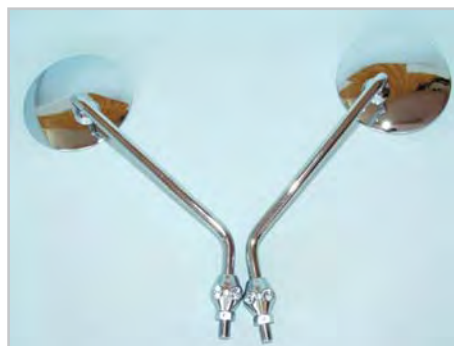
HONDA MR52L & MR52R O.E No L/H: 88120-443-620/621 / 88120-KB7-000 O.E No R/H: 88110-443-620/621 / 88110-KB7-000 TYPE: Convex HEAD: Round / Chrome STEM: Chrome FITTING: Handlebar THREAD: 10mm FIXING CENTRE:
