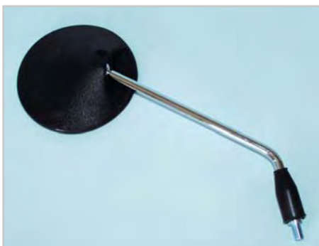
HONDA MR10 O.E No L/H: 88110-GB4-000 O.E No R/H: 88110-GB4-000 TYPE: Convex HEAD: Round / Black STEM: Chrome FITTING: Handlebar THREAD: 8mm FIXING CENTRE:
