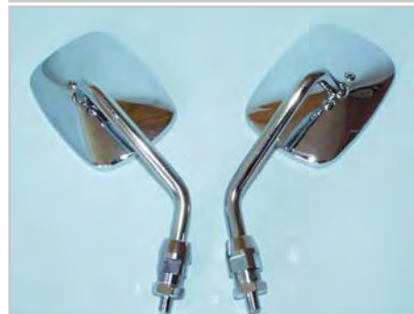
TRIUMPH MIR233L & MIR233R O.E No L/H: T2300523 O.E No R/H: T2300524 TYPE: Convex HEAD: Chrome STEM: Chrome FITTING: Handlebar THREAD: 10mm FIXING CENTRE:
